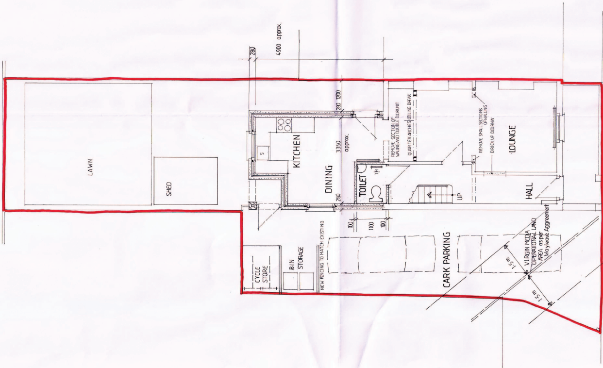
GROUND FLOOR PLAN — AS PROPOSED — 1:50
